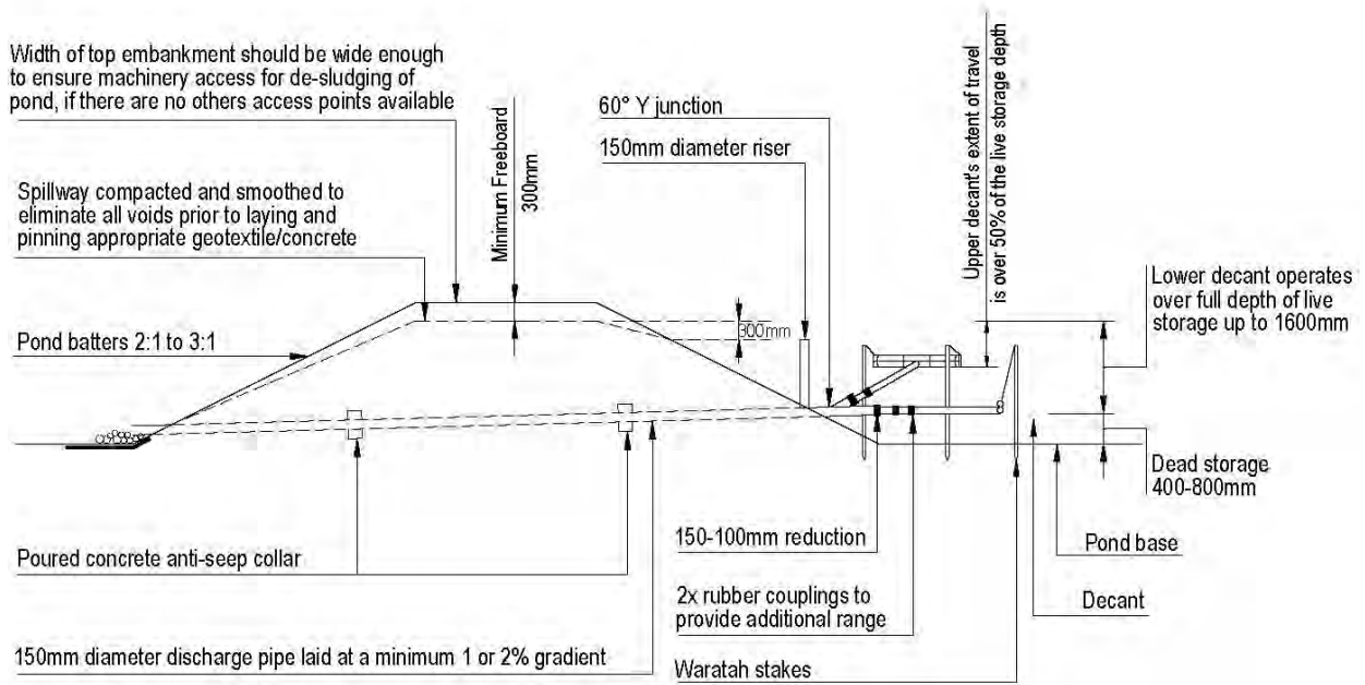
Cross - section
