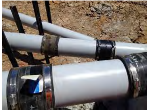
Figure 77: Steel strapping used to attach decant system to horizontal pipework
