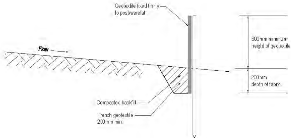
Cross section
