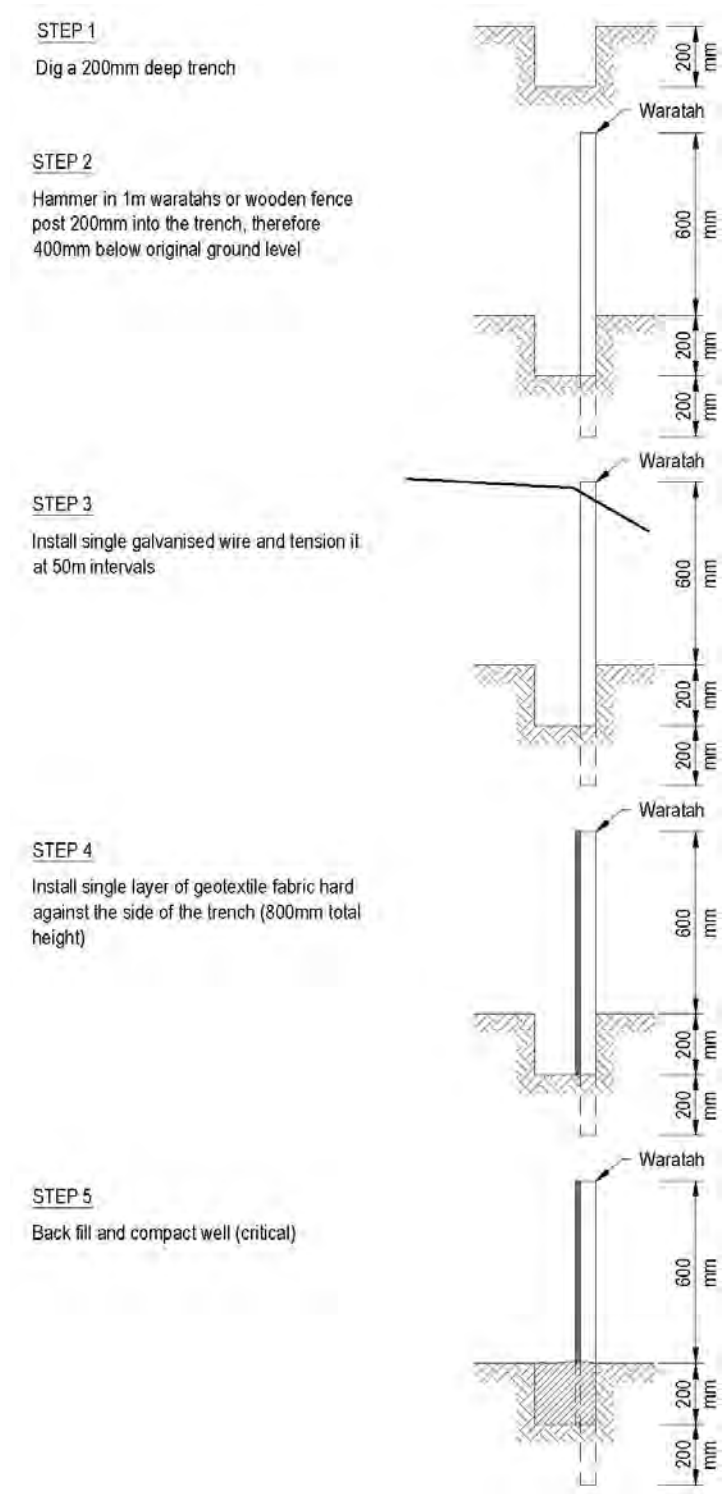
Figure 84: Step-by-step installation of a silt fence
