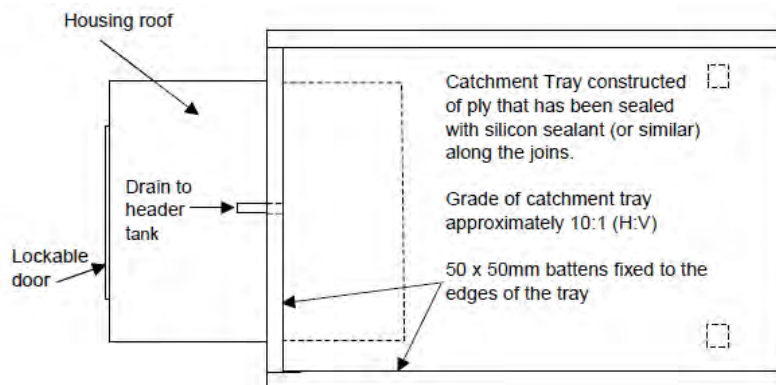
Figure 102: Rainfall catchment tray
