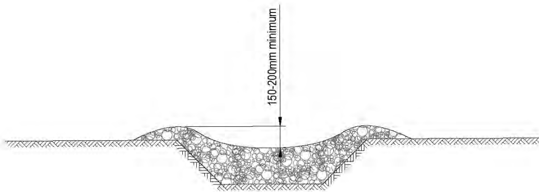
Cross - section
